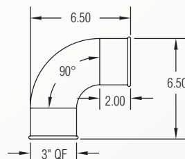
3" 90° Elbow (1.0CLR)
