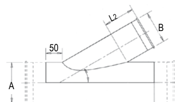
Wcinka Quick-Fit 30°
