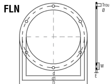
Brides FLN
