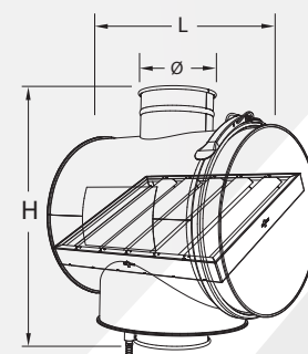
Vertical Installation
