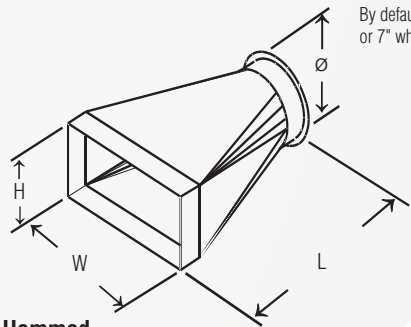
Hemmed or Raw Rectangular End Type
