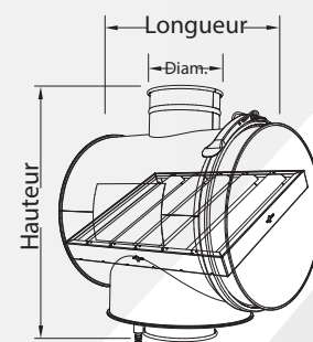
Installation verticale
