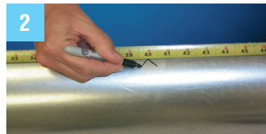
2 Mark distance to be spanned less 4".
