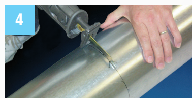
4 Drill access hole, then cut Pipe with saw.
